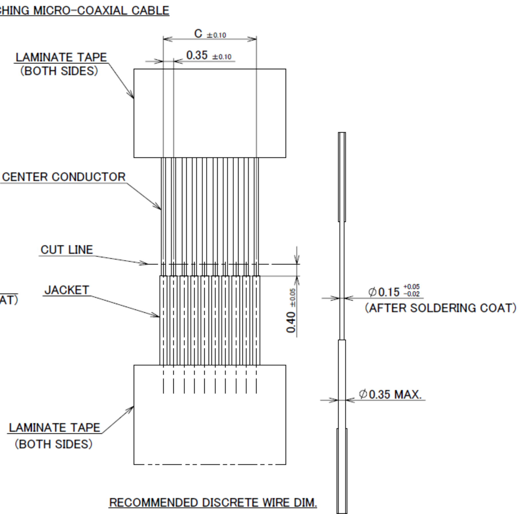
DISCRETE WIRE AWG# 36
